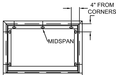
TYPICAL ELEVATION WITH FASTENER SPACING
